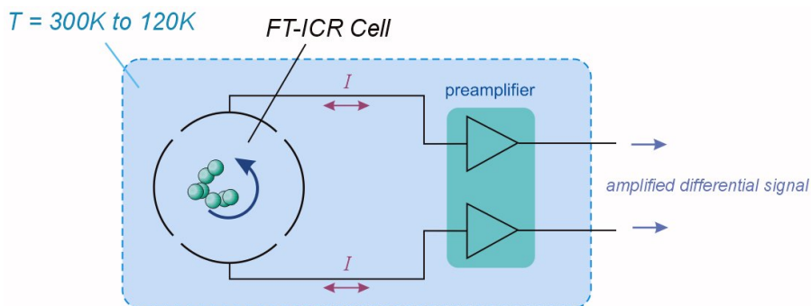
Fig. 1a: Typical Application: Differential Signal Detection in FT-ICR Cells
