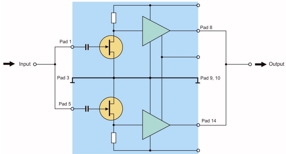
Fig. 16: Connection scheme for “single channel” operation, used to obtain data of figures 14 and 15.
