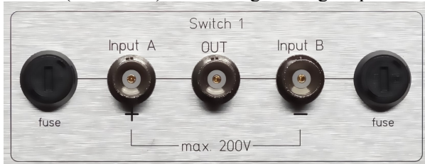
fig. 4.4: BNC sockets for high voltage inputs and output; note that voltages higher 500V require SHV sockets and note that in case of the HS-2000 version, the input fuses are located internally (replaceable fuse: 32mA)
