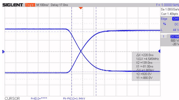
fig. 4.6 positive and negative voltage step of 2000V with medium capacitive load ( C = 100\text{pF} ), corresponding to about 1m of standard SHV cable (RG58) or 2m of low-capacitance cable; transient rise time (10% to 90%) is about 230ns each (grid: 100ns/div).
