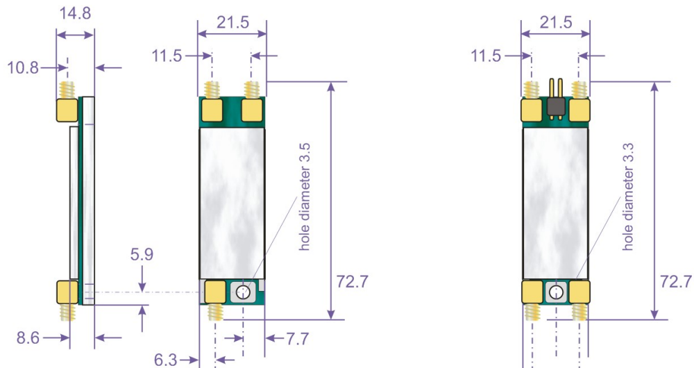
Figure 18c, d: Outline dimensions 1-channel version and 2-channel version with SMA terminals
